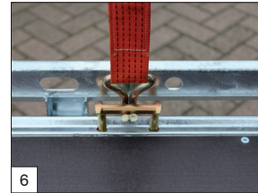
Standard: the fixing points have a capacity of 1000 daN (kg.) each.
