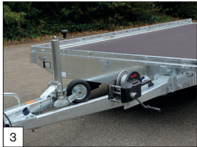
Standard: a robust, adjustable winch with support in front.
