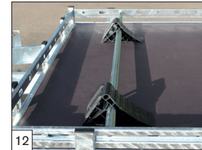
Option: adjustable wheel chock model Combi Protect Rail and 2 black wheel chocks.
